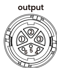
Female connector
