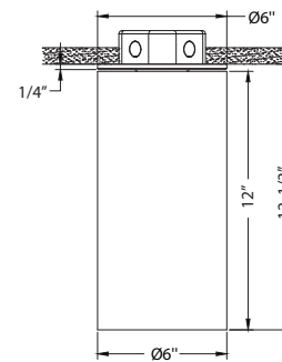
Surface Mount
