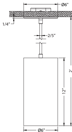
Conduit Pendant Mount (with 1' stem)
