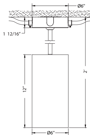
Conduit Stem Mount (with 1' stem)
