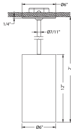
Stem Mount (with 1' stem)
