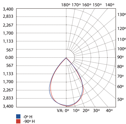
CLI6A-40W-T1 @4000K 70°
