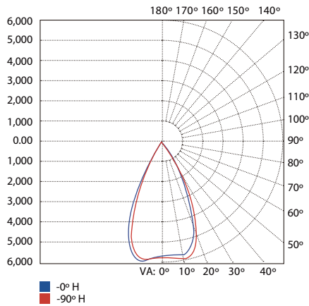
CLI6A-40W-T1 @4000K 50°
