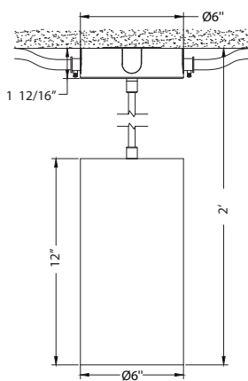
Conduit Pendant Mount (with 1' stem)
