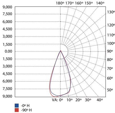
CLI6A-40W-T1 @4000K 40°
