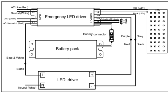
Wiring diagram (Maintained)
