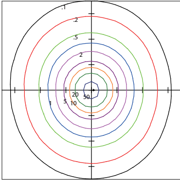
ISOCANDELA PLOT
