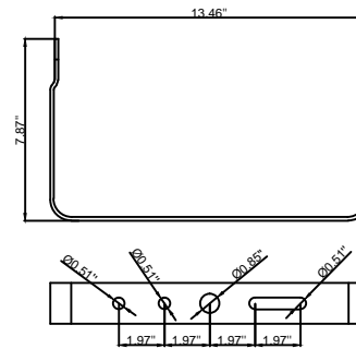
MYK-AR-G2B ( \pm 160^\circ )
