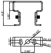
MTN-AR-G2 ( \pm 90^\circ )
